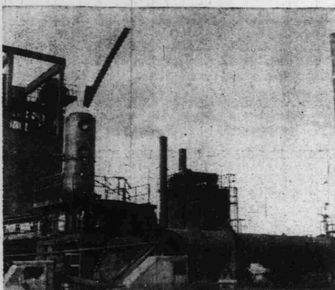
NEW SCRUBBER — Pictured is the new wet system scrubber to remove manganese ore dust from an exit gas stream at AMPOT. This dust, as can be seen from the stack beside the new scrubber, was a small contributor to air pollution. The new scrubber is guaranteed to meet regulations of the Los Angeles Air Pollution Control District insofar as dust emissions into the atmosphere are concerned. This installation brings expenditures on this dust problem to around $40,000 in the past ten years.
