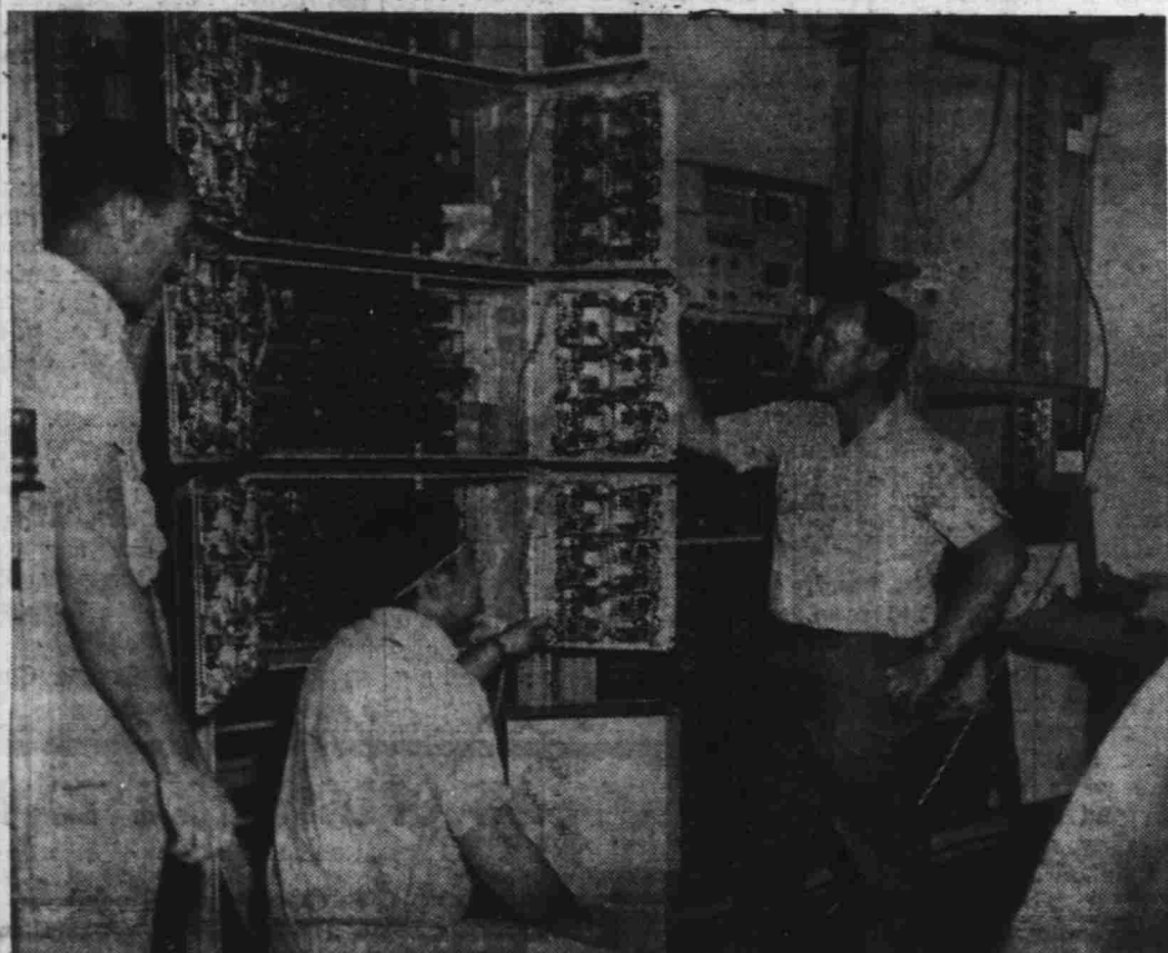
MAKING THE FINAL CHECK of the new register senders which will be used to handle long distance calls for nation-wide dialing and which will permit Henderson subscribers to participate in the Extended Area Service program with Las Vegas and Boulder City. Shown in the photograph left to right, are S. W. Roberts and D. P. Ross, both of the Stromberg Carlson company and Dick Pryor of the Henderson Telephone Company.
