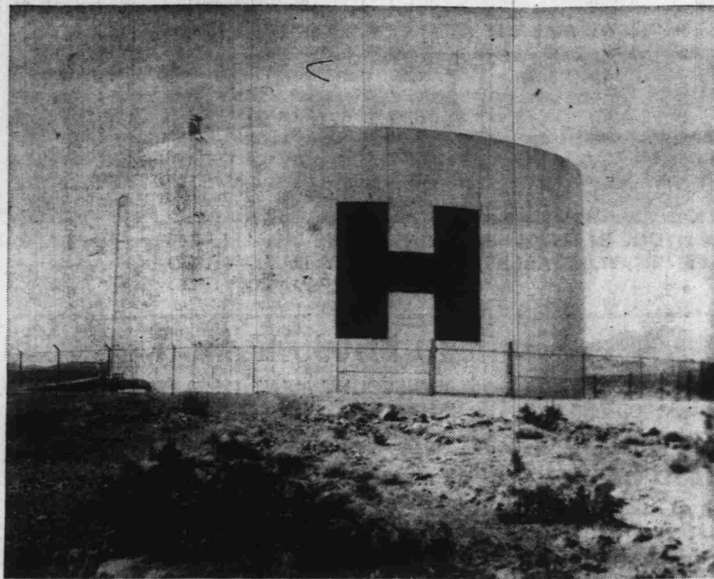
STORAGE TANK — Here is the big tank on the hill in which the water is stored to provide gravity pressure to the homes below. This tank holds one million gallons and is filled three and a half times a day throughout the year. The huge "H" stands for Henderson, not 'ot.
